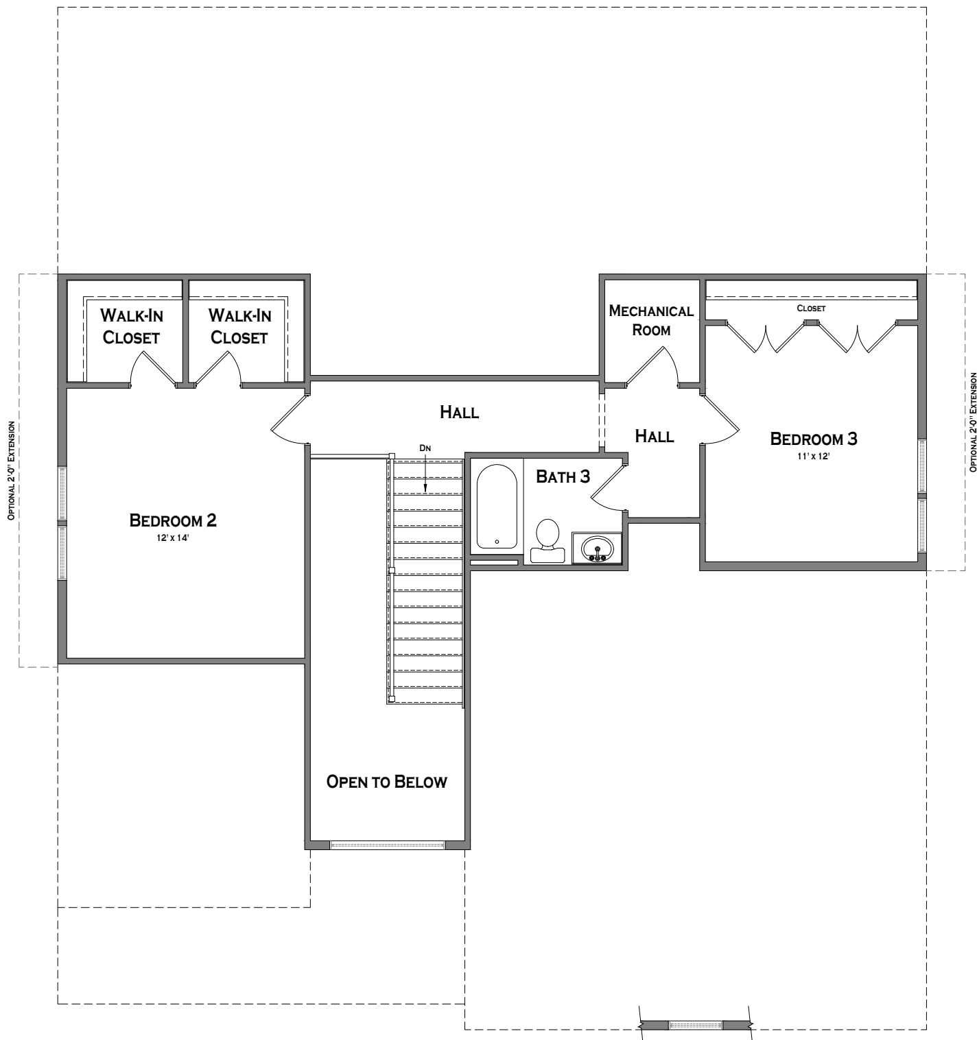
SECOND FLOOR
