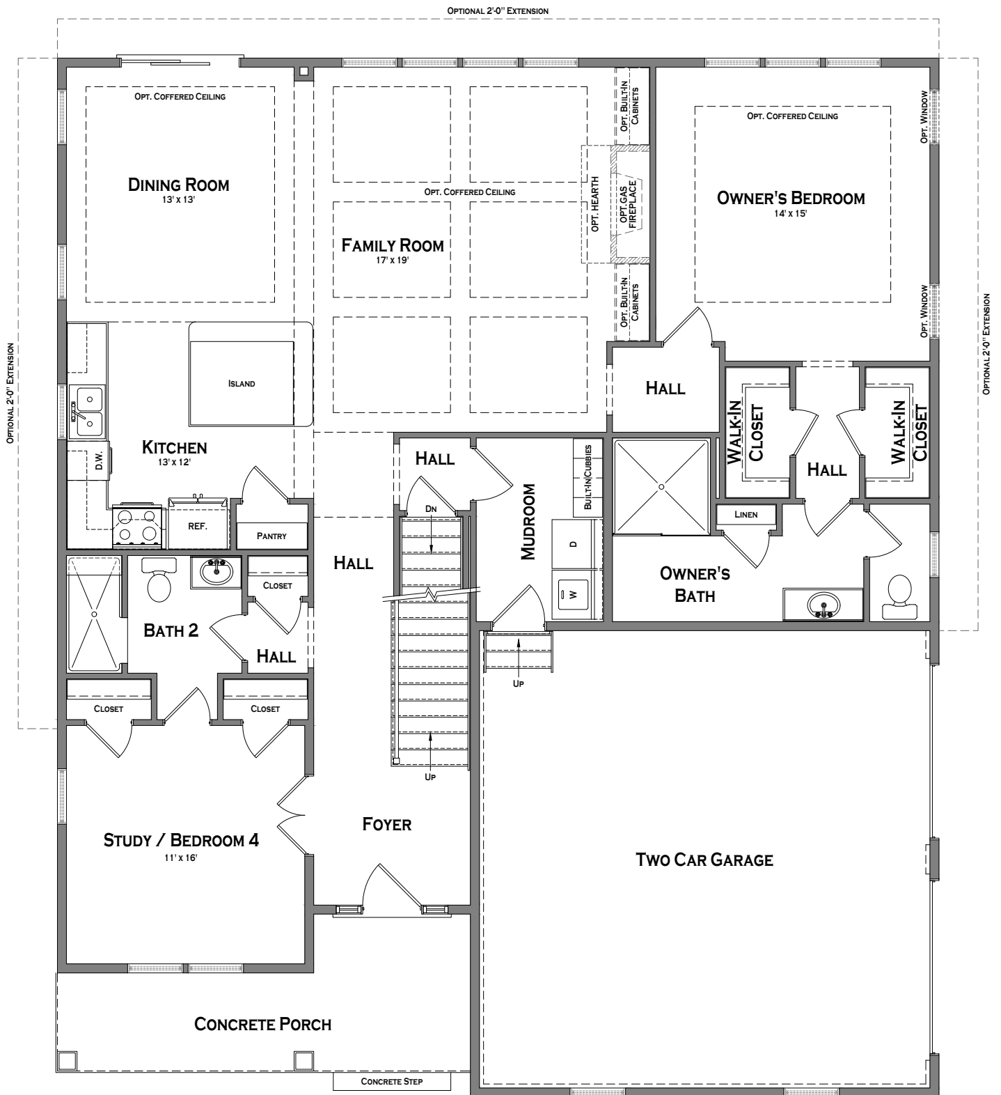
FIRST FLOOR
