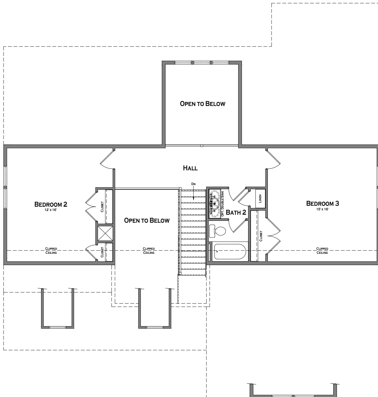
SECOND FLOOR
