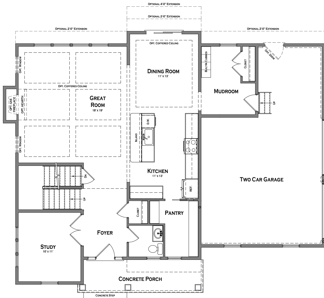
FIRST FLOOR
