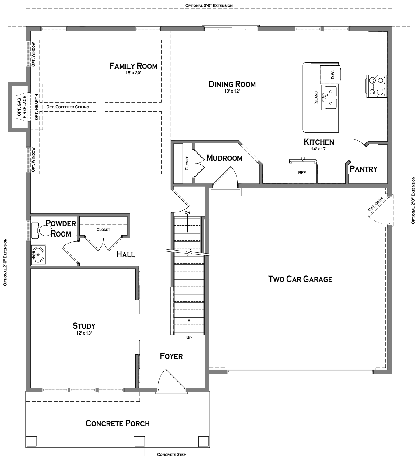
FIRST FLOOR
