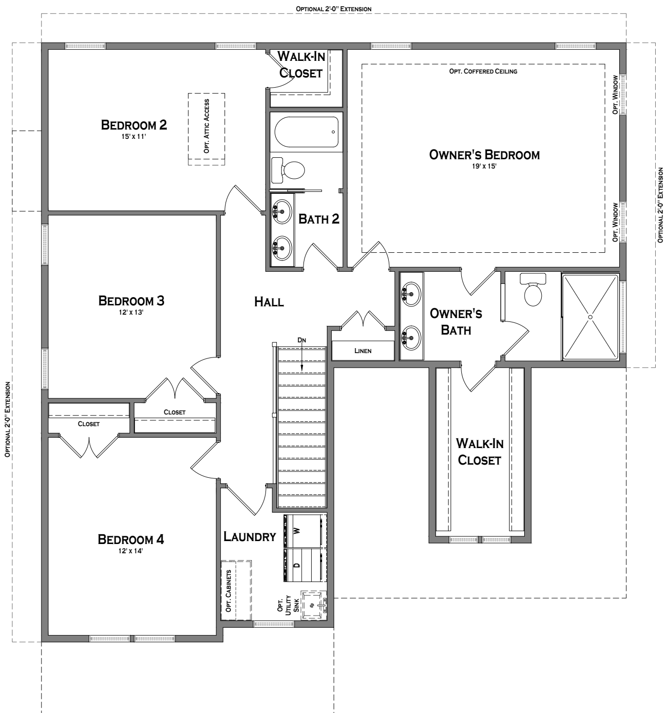
SECOND FLOOR
