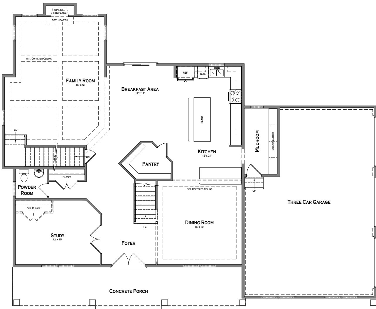
FIRST FLOOR
