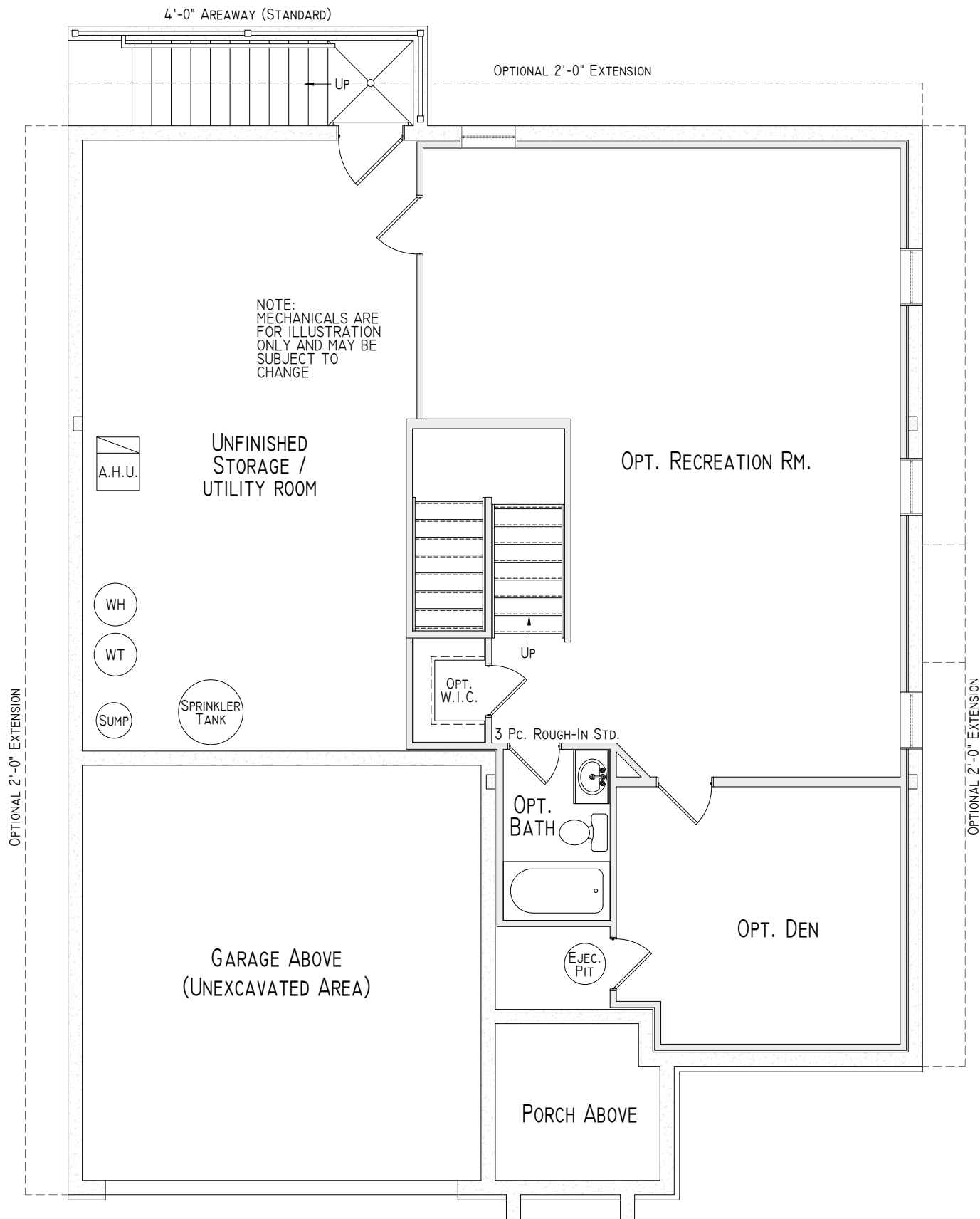
Foundation Plan
