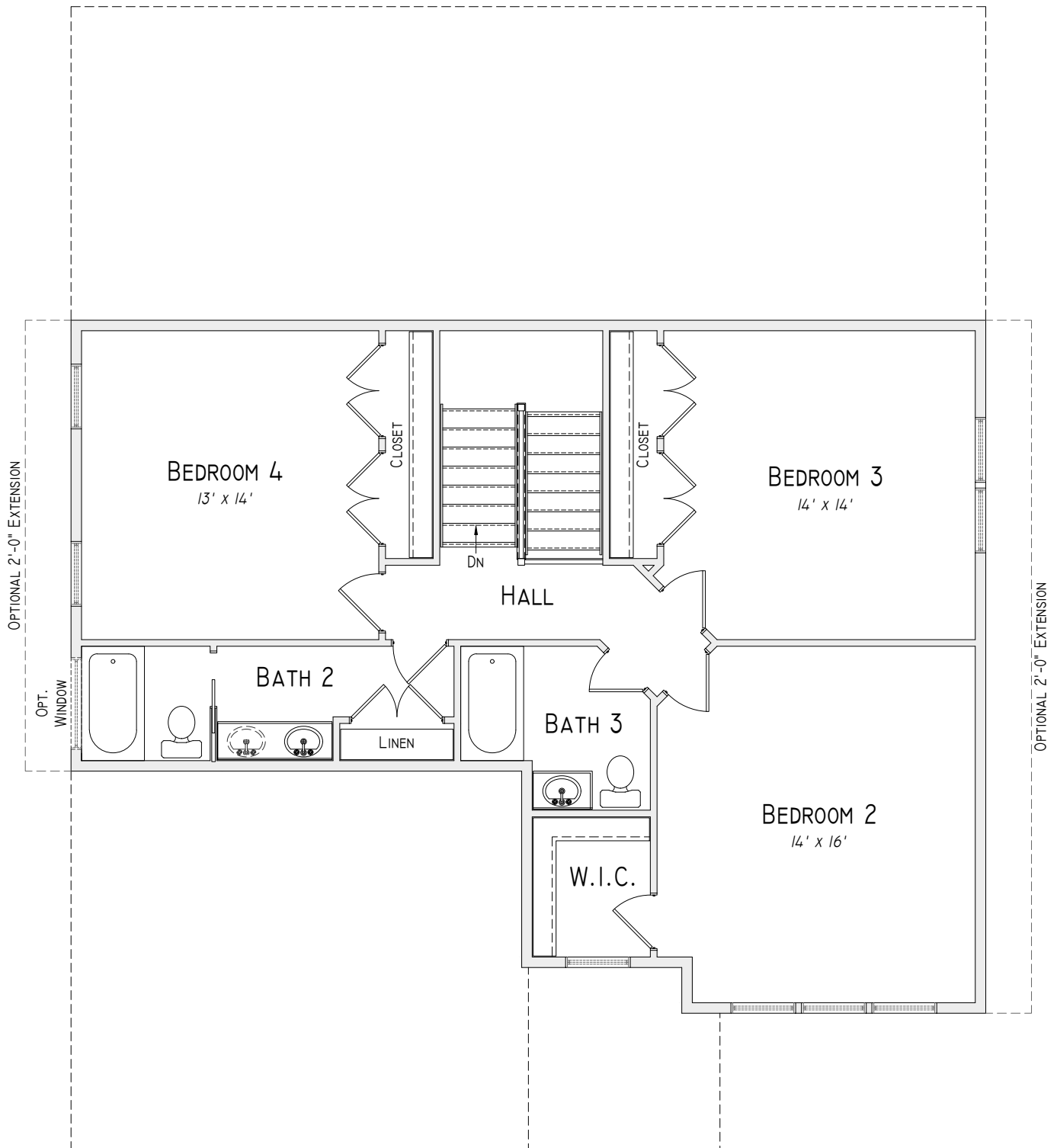
Second Floor Plan w/ Optional Bath 3
