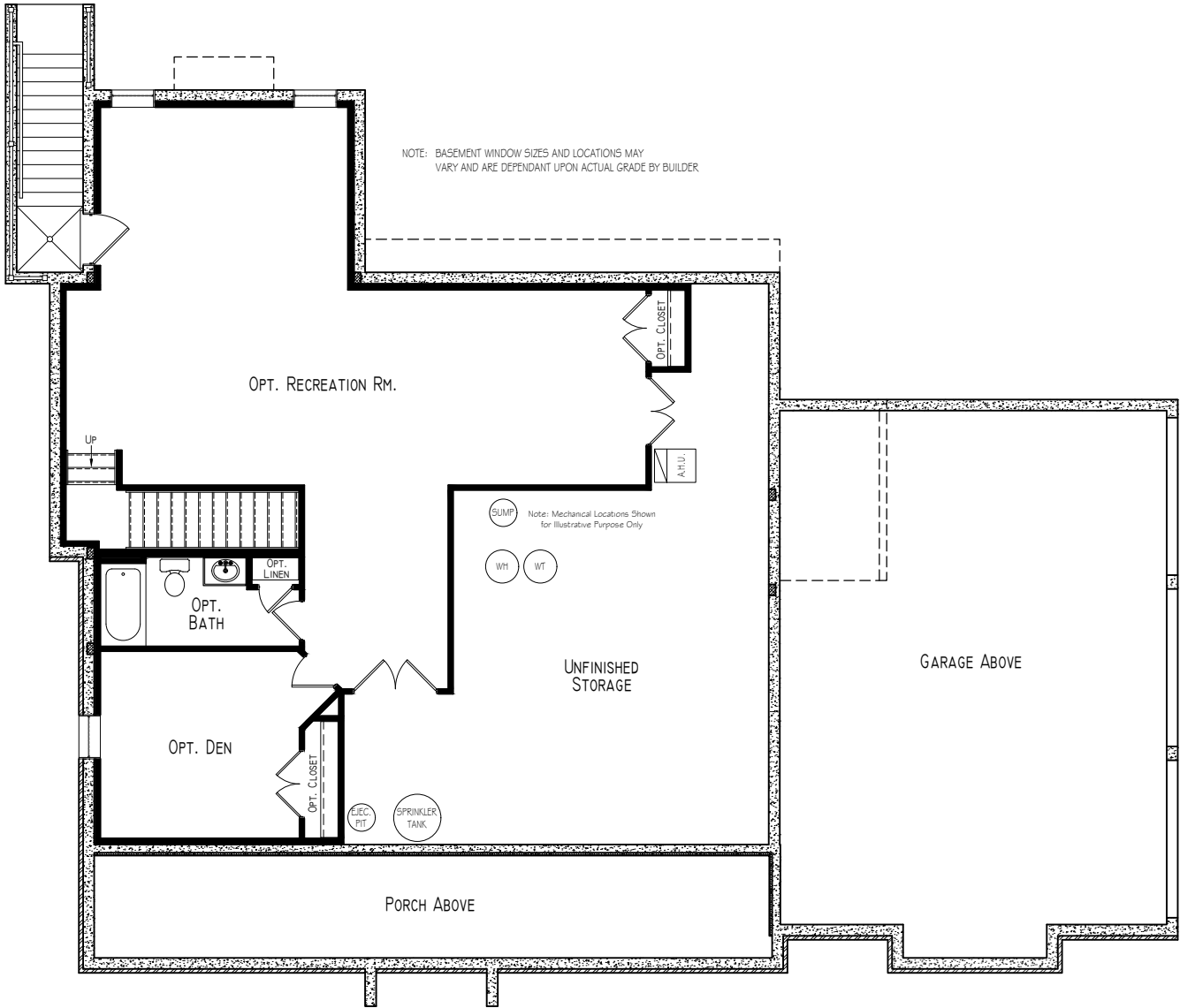
Foundation Plan
