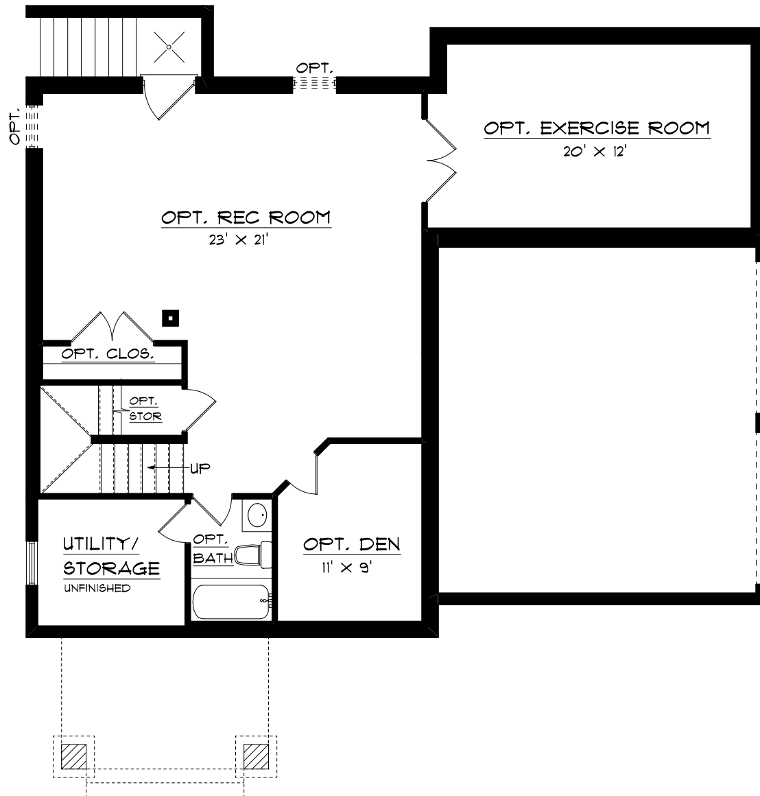
OPTIONAL FINISHED BASEMENT PLAN @ ELEVATION #3
